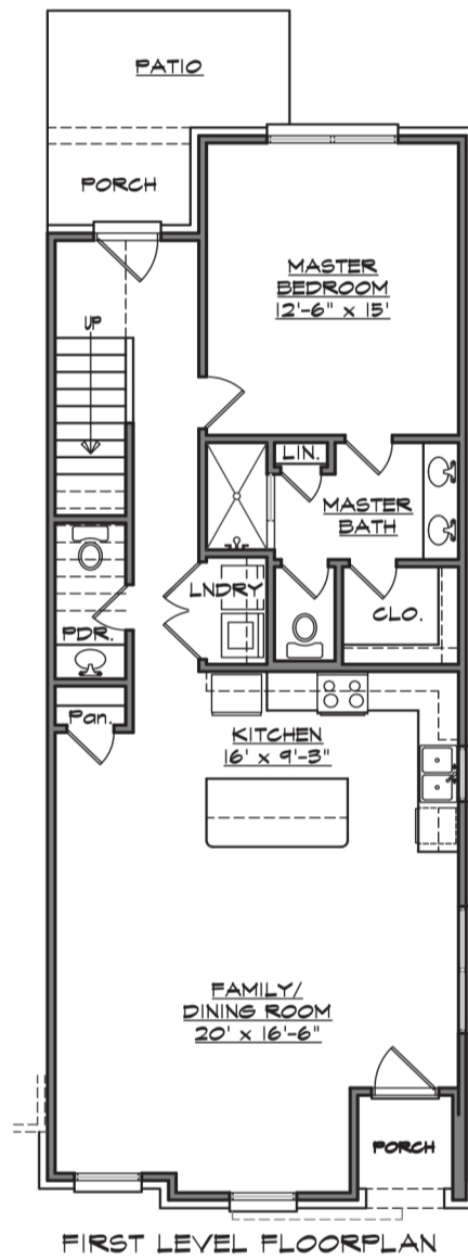
FIRST LEVEL FLOORPLAN
